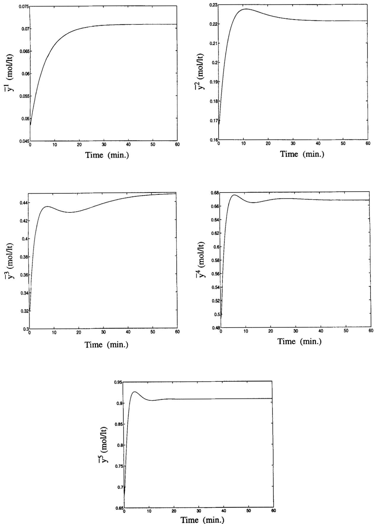
Figure 9. Output profiles for a 30% increase in the reference inputs-discretization-based controller.
