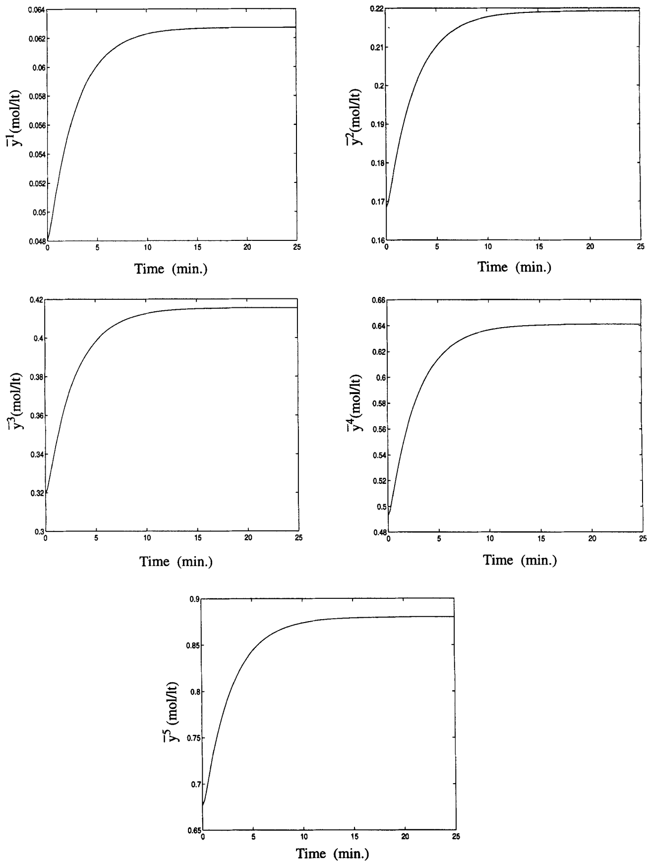
Figure 11. Output profiles for a 30% change in reference inputs—jacket inlet flow rates are used as the manipulated inputs.
