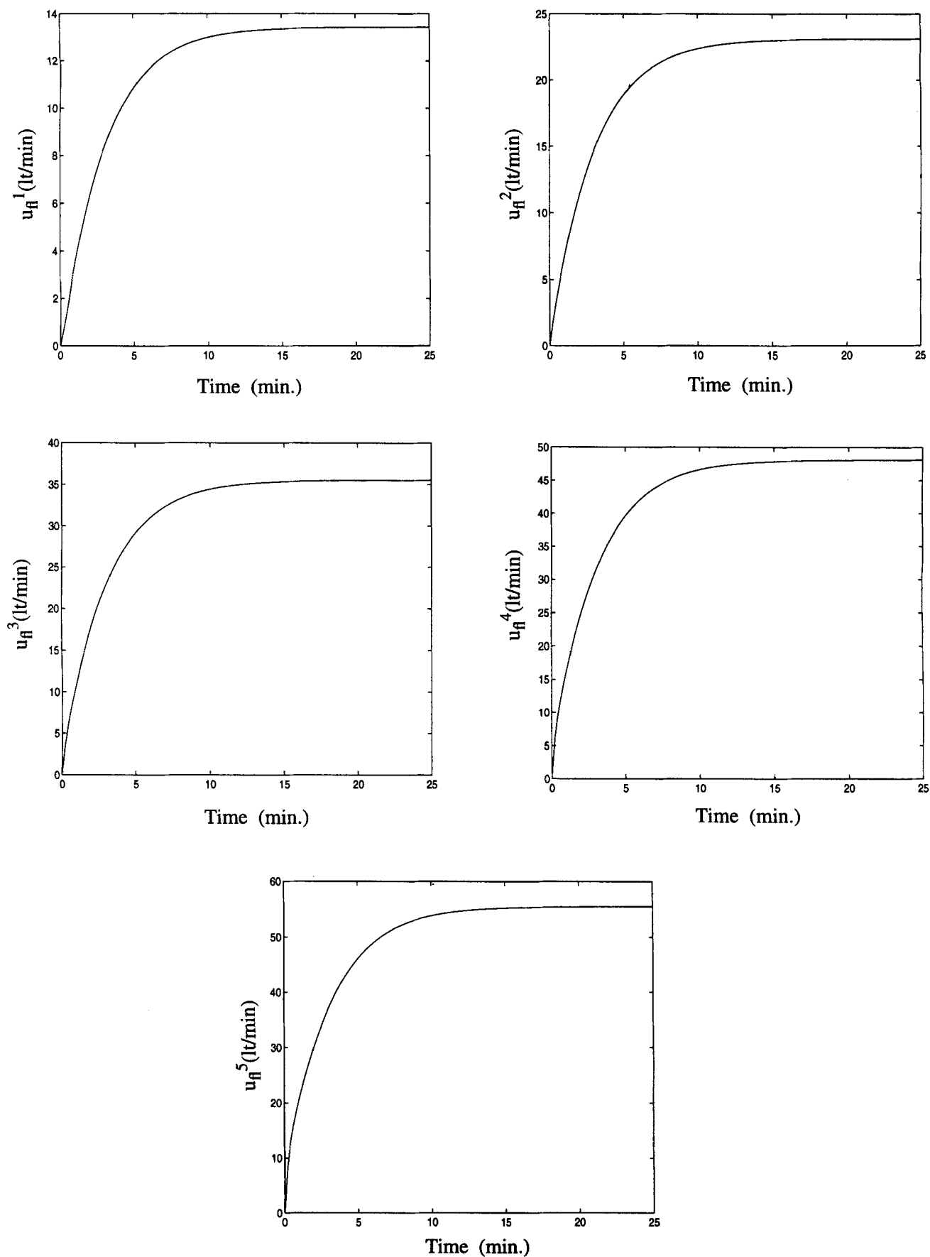
Figure 12. Profiles of jacket inlet flow rates for a 30% increase in reference inputs.
