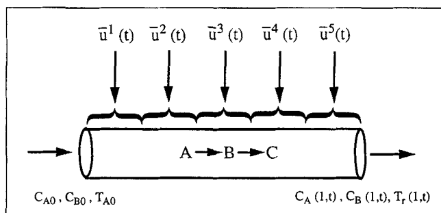
Figure 4. Specification of the control problem for the plug-flow reactor.
